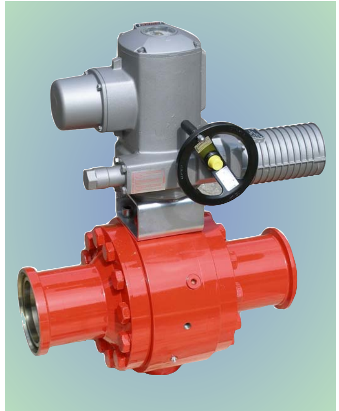
metallisch dichtender ASC KH Sonderflansch metall seat ASC ball valve special connection
